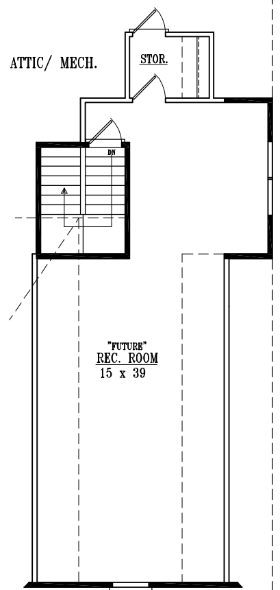
SECOND LEVEL FLOOR PLAN
