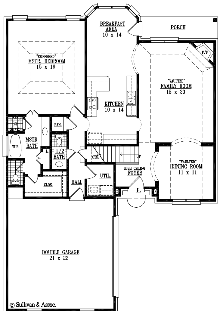
FIRST LEVEL FLOOR PLAN
