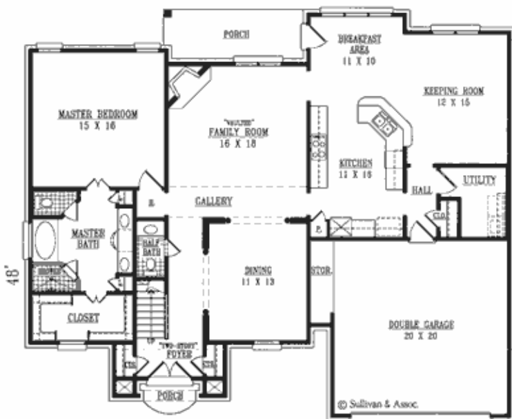
FIRST LEVEL FLOOR PLAN
